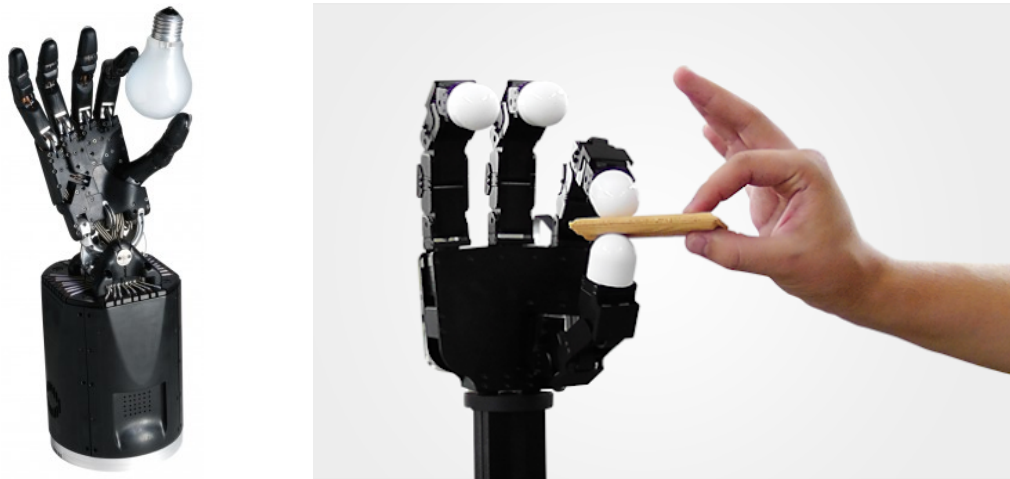
Figure 2.3 - Dexterous hands. Left: the Shadow Dexterous Hand . Right: the Allegro Hand .
