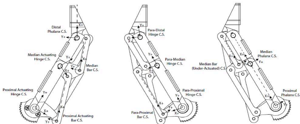
Figure 2.6 - A clever mechanical linkage allows the underactuated Robotiq 3-fingered gripper to comply to an object being grasped.
